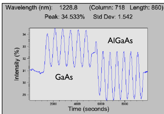
Figure 2: Pyrometric interference oscillations at 1228nm for GaAs/AlGaAs deposition.
